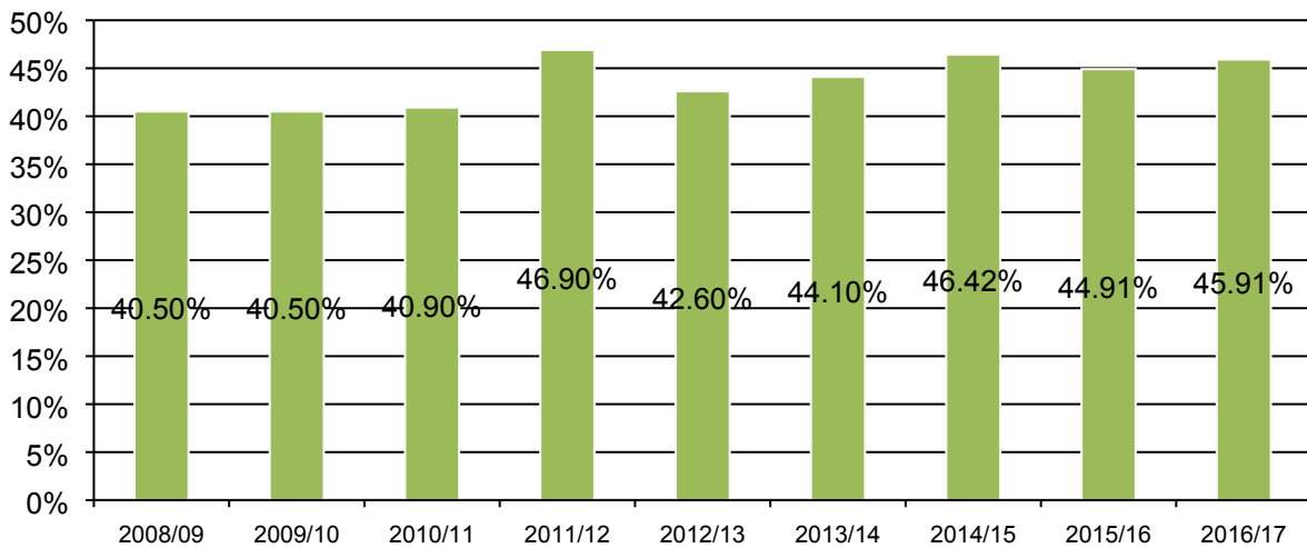
NI 192: Dry Recycling and Composting as Percentage of Household Waste (2016/17: at Aug 2016)
